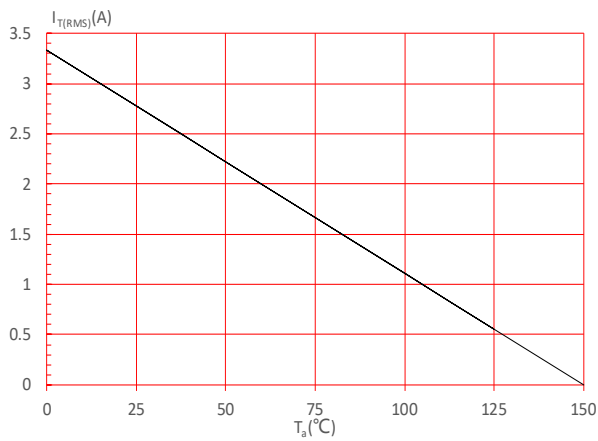
FIG.5: On-state characteristics
