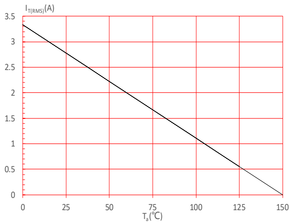
FIG.5: On-state characteristics
