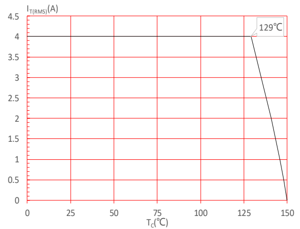
FIG.4: On-state characteristics
