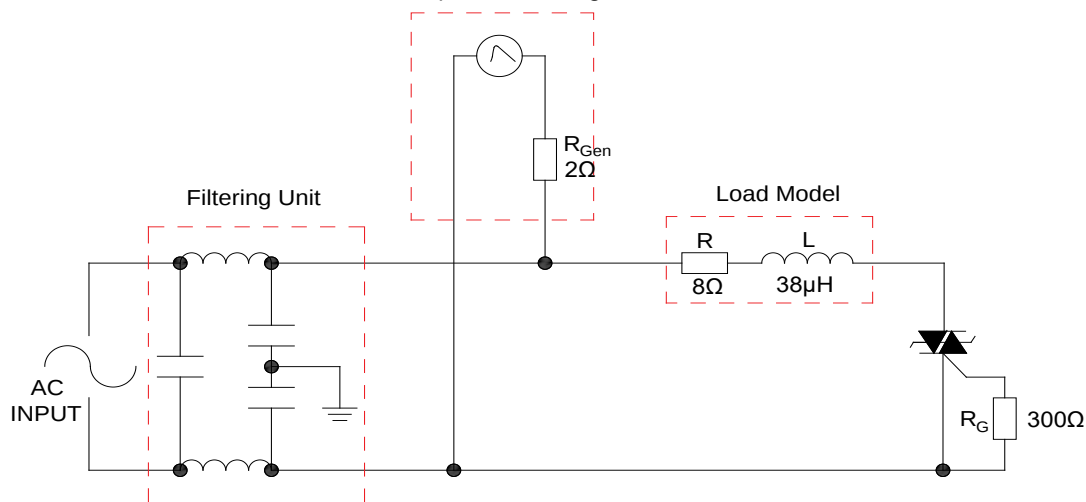
IEC61000-4-5 Standards Surge Generator 1.2/50 \mu S voltage surge 8/20 \mu S current surge
