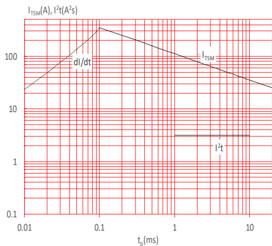
FIG.5: Non-repetitive surge peak on-state current for a sinusoidal pulse with width t_p < 20ms , and corresponding value of I^2t ( dl/dt < 100A/\mu s )
