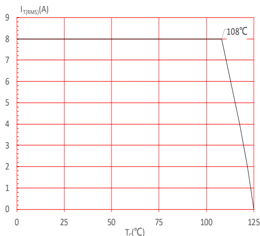
FIG.4: On-state characteristics
