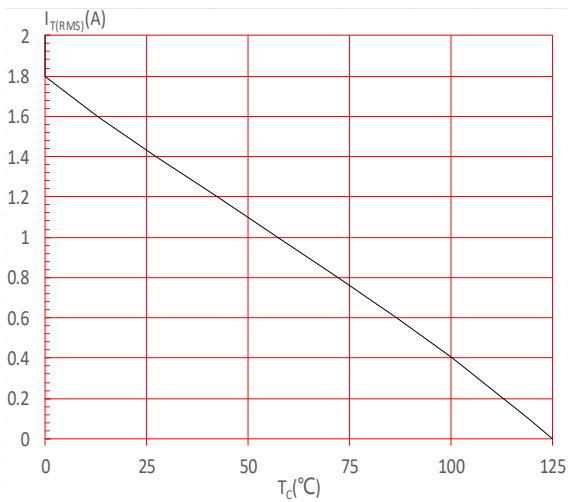
FIG.4: On-state characteristics
