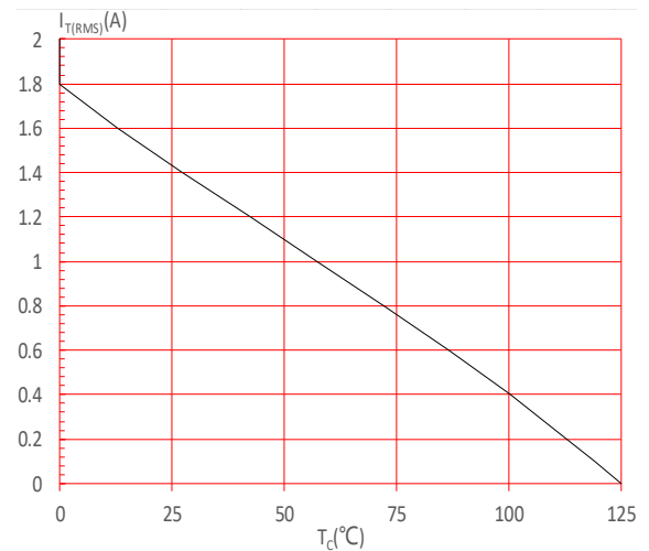
FIG.4: On-state characteristics
