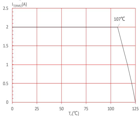
FIG.4: On-state characteristics
