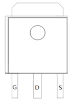
Pin Assignment
